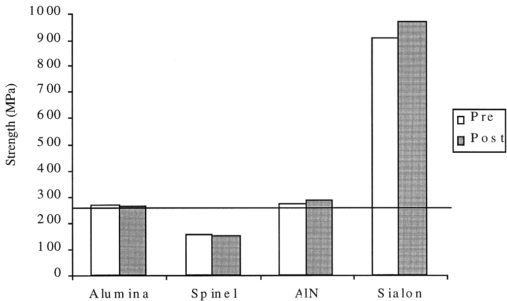
Fig. 3. Effect of 0.1 dpa fast neutron dose on flexural strength.
