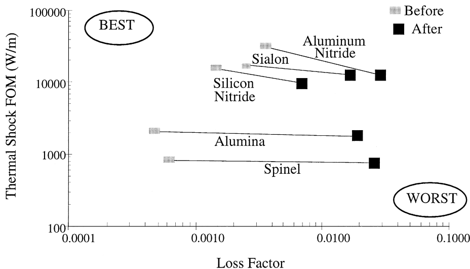
Fig. 5. Window performance parameters before and after a fast neutron dose of 0.1 dpa.
