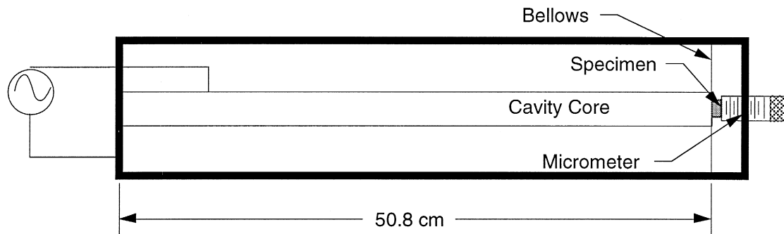
Fig. 2. High resolution loss tangent measurement cavity.
