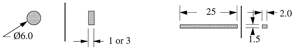
Fig. 1. Thermal/dielectric and mechanical specimens used in irradiation of ceramic materials (dimensions in mm).
