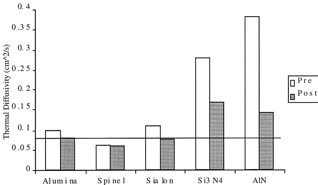
Fig. 4. Effect of 0.1 dpa fast neutron dose on thermal diffusivity.
